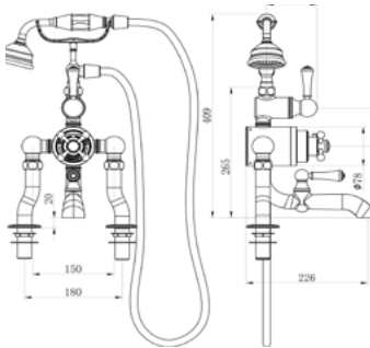
TR-BT-UK16 TRADITIONAL CHROME THERMOSTATIC BATH TAPS
