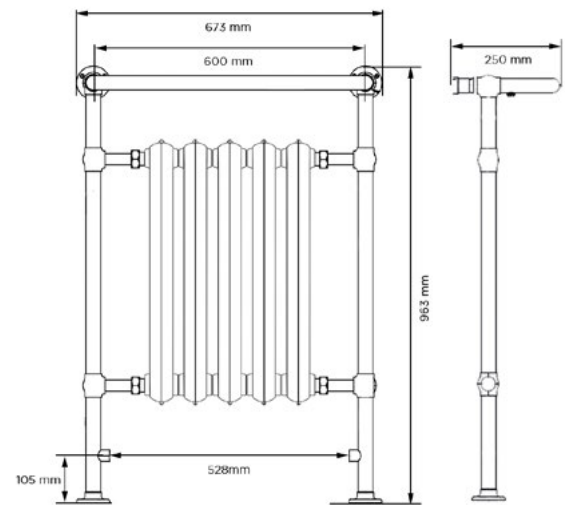
Column Towel Radiator in Copper with Farrow & Ball Pitch Black Colour Match Insert
